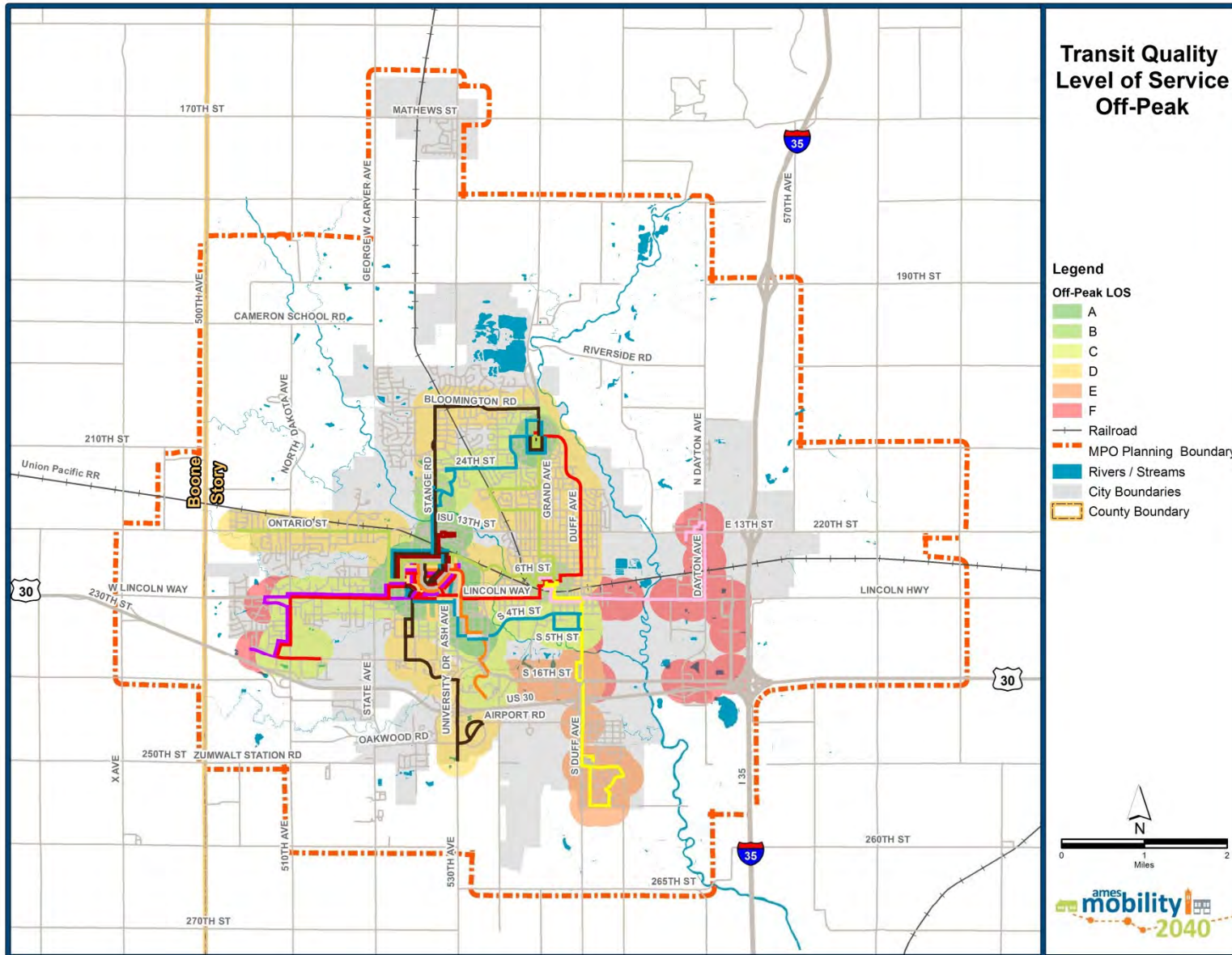
Figure 47. Transit Quality Level of Service - Off-peak
