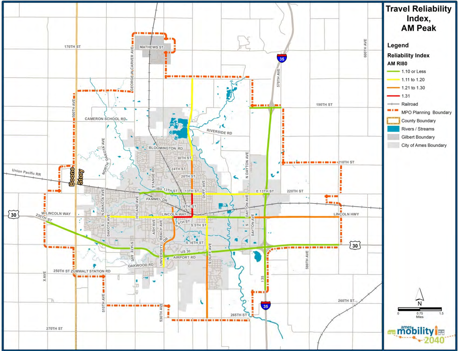
Figure 37. Travel Reliability Index, AM Peak
