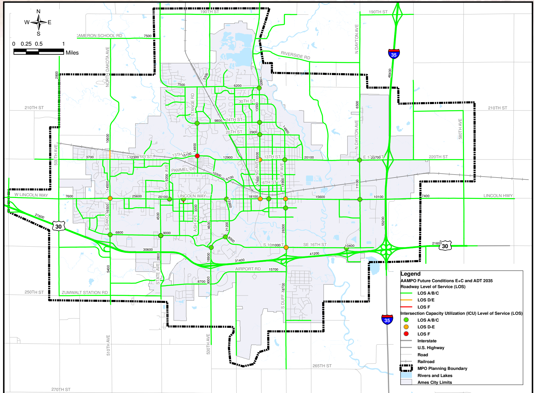
FIGURE 5.9. 2035 E+C AVERAGE DAILY TRAFFIC VOLUMES, INTERSECTION LOS AND ROADWAY SEGMENT LOS
